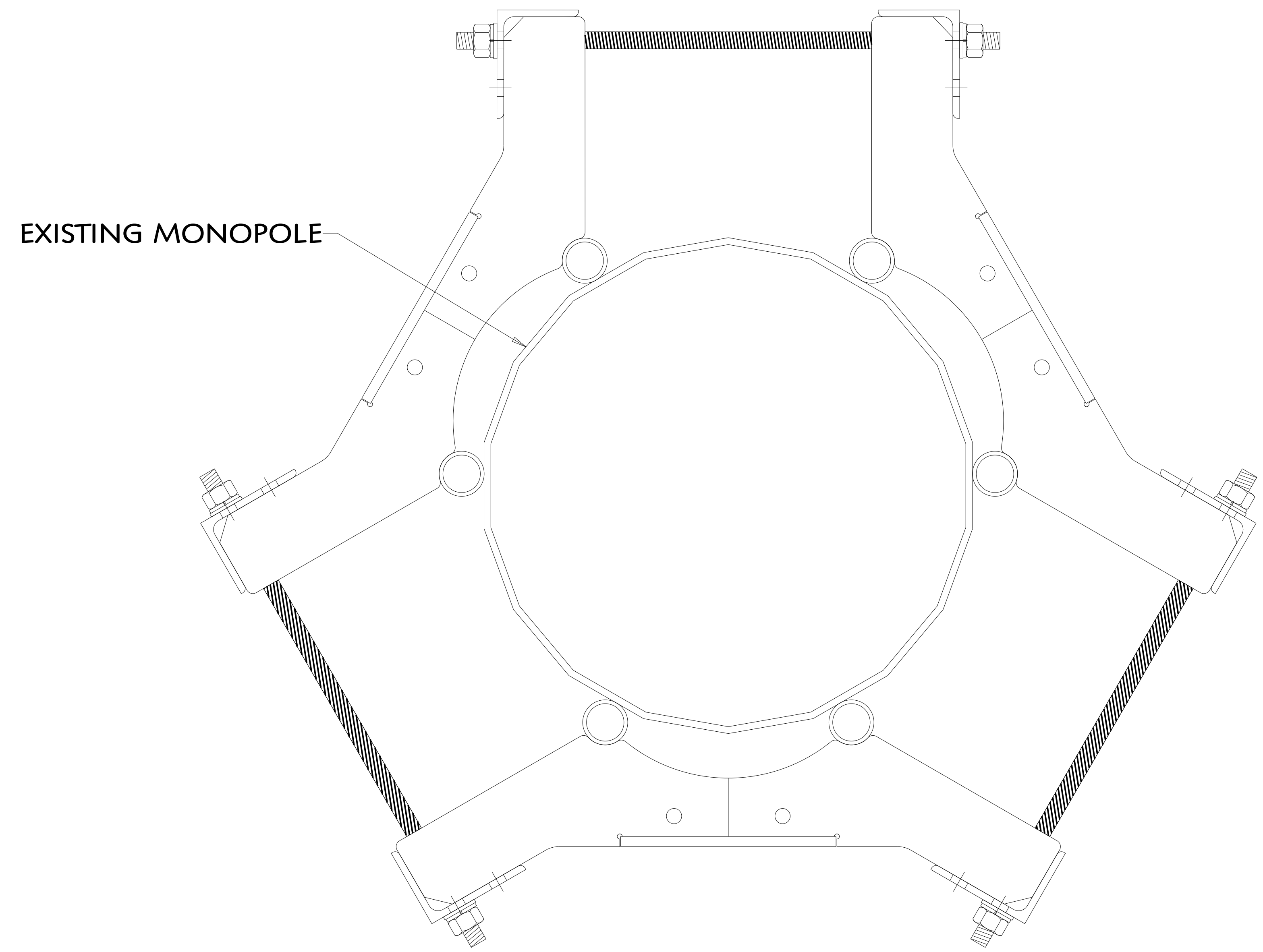
PLAN VIEW MONOPOLE COLLAR MOUNT ASSEMBLY
